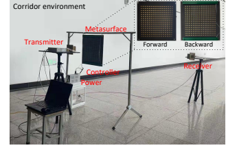
Figure 12: Evaluation setup.
